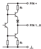
picture 3: transistor output
