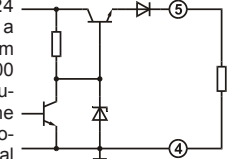
picture 4: Alarm output
