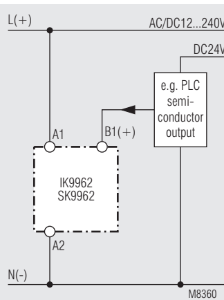
Connection with 2 different control voltages
