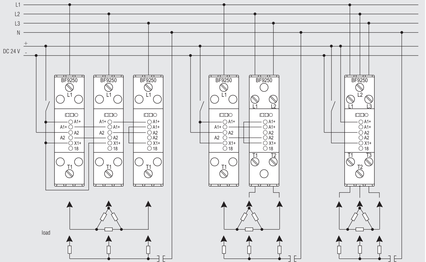
3-phase load switched by 3 single-pole semiconductor contactors
