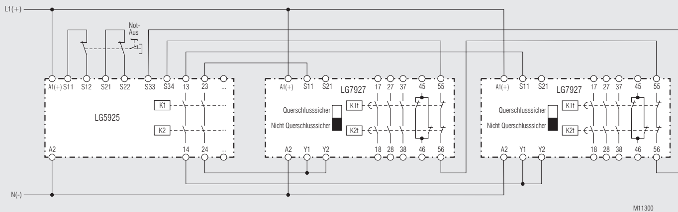
LG 5925 with two LG 7927, non cross fault detection, suitable up to SIL2, Performance Level d, Cat. 3
