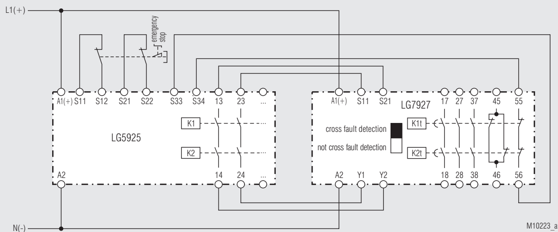
LG 5925 with LG 7927, cross fault detection, suitable up to SIL2, Performance Level d, Cat. 3
