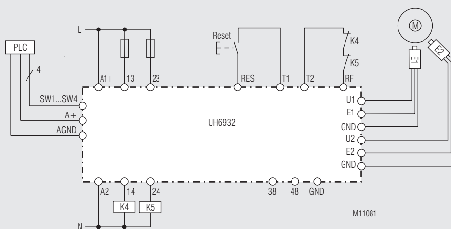
Standard connection with UH6932/_ _1, Suited up to SIL3, Performance Level e, Cat. 4
